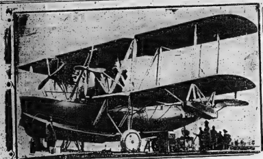
Shown is the first three-motored amphibian plane, ever built and which recently passed all tests. The plane has been turned over to the British Air Ministry. It is a four with two 200 h. p. "Reliance" "Lodge" engines and is one of the first of planes being developed for the civil aviation department of the air ministry for commercial purposes. The amphibian is designed to carry twelve passengers a pilot and an observer. It is capable of taking off and landing on land or water.
